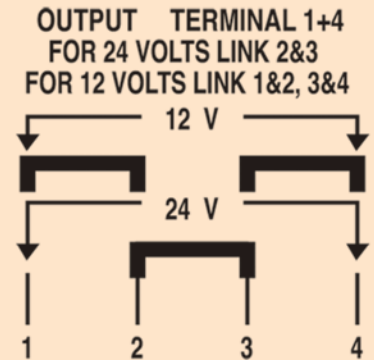
Typical series/parallel connections
