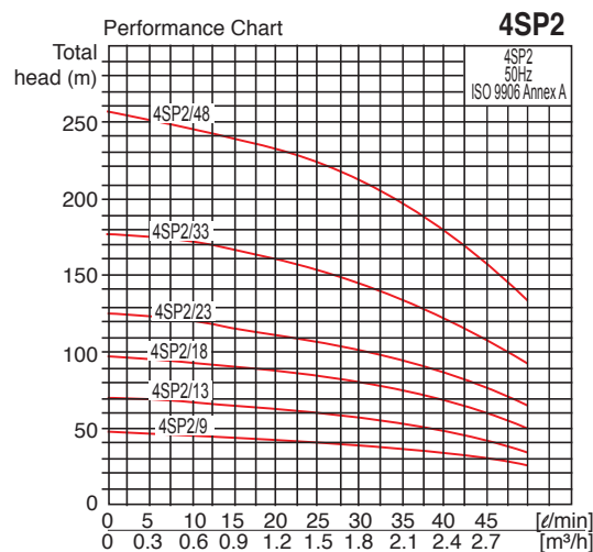
4" STAINLESS STEEL DEEP WELL SUBMERSIBLE PUMPS
