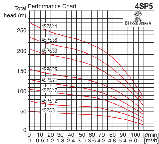
4" STAINLESS STEEL DEEP WELL SUBMERSIBLE PUMPS
