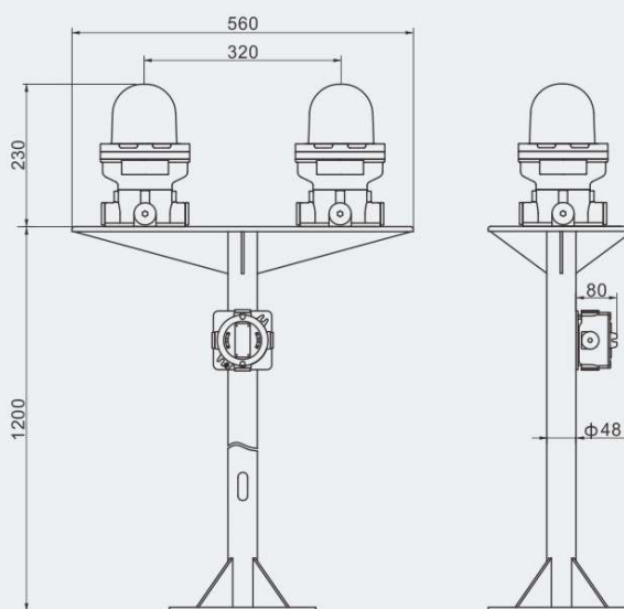
Drawings of main (spare) caution spotlight fittings
