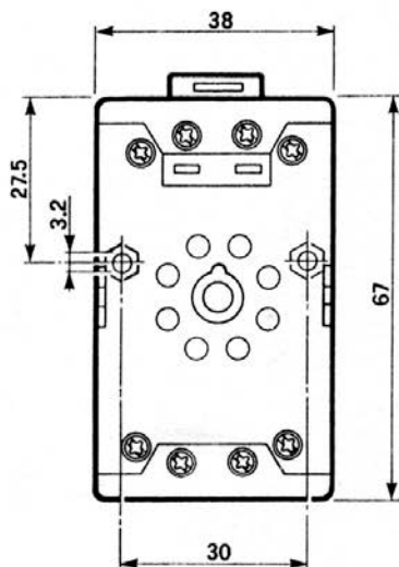
ZVO (8-pin)
