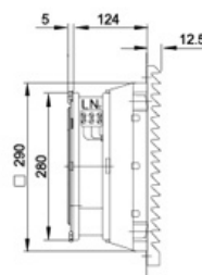
Fans and filters FKL 6626.230-D
