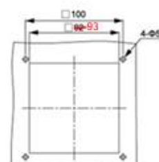
Drawing FKL 6621....
