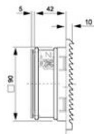
Fans and filters FKL 6621.230
