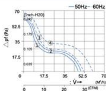
Performance FKL 6621....
