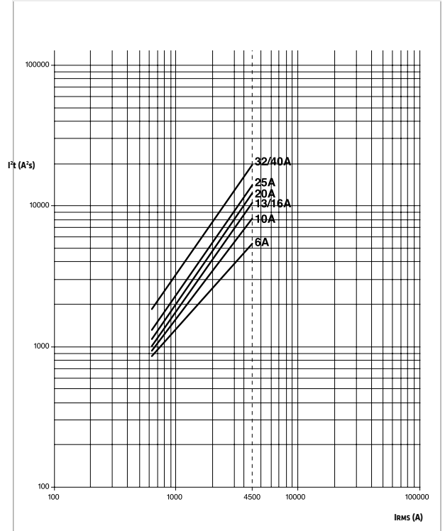
MT 45 - 2P 400V C characteristic
