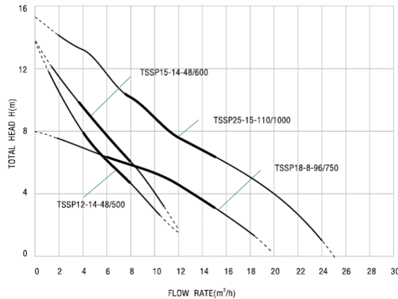
Performance Curve
