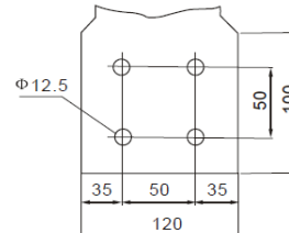
3150~4000A
