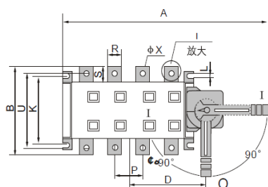
YGLZ1-125~1600A Direct operation
