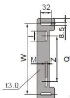
Installation size of handle seat outside board
