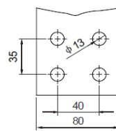
3150~4000A
