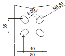
1250~2500A
