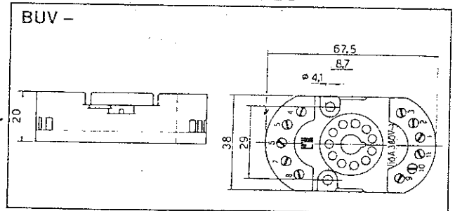
11-pin screw terminal socket for panel board mounting DIN 46277 - rail mounting
