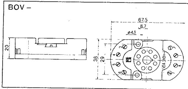
8-pin screw terminal socket for panel board mounting DIN 46277 - rail mounting
