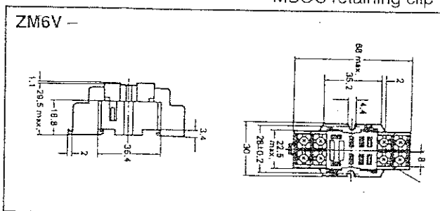
Screw terminal socket for relay Type D6/SL ZM6CS: for printed circuit sockets:
