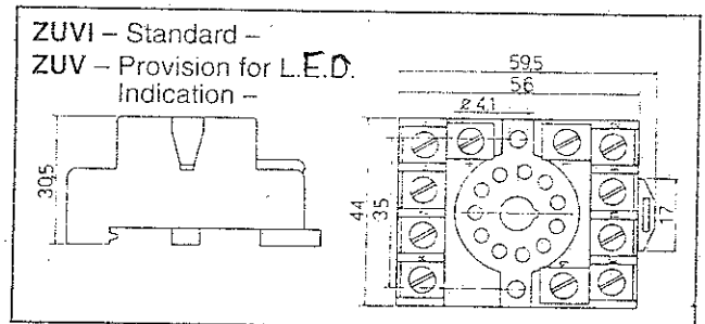
11-pin screw terminal socket for panel board or DIN 46277 - rail mounting
