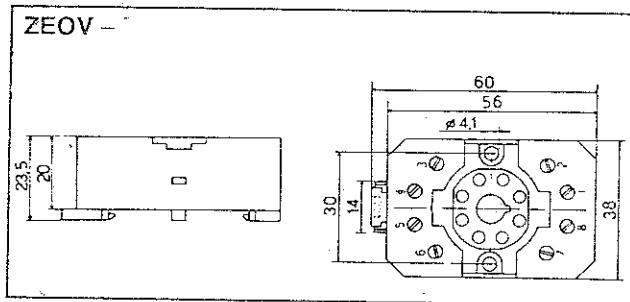
8-pin screw terminal socket for panel board or DIN 46277 - rail mounting
