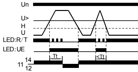
Overvoltage, non-latching mode
