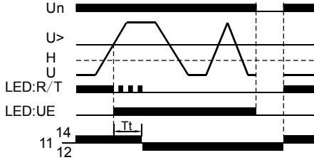
Overvoltage, latching mode
