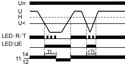
Undervoltage, non-latching mode
