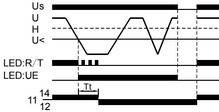
Undervoltage, latching mode
